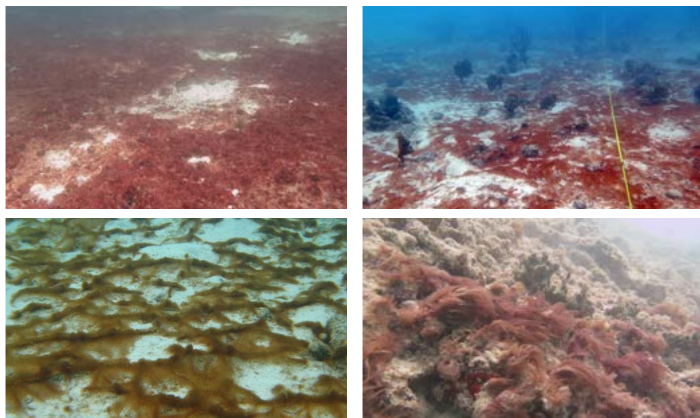
FIGURE 13: Examples of benthic communities dominated by cyanobacteria and turfalgae. The high production of organic material by such communities in combination with land-based factors (e.g., sewage, nutrients) creates "microbialized" landscapes with high oxygen demands which can lead to the formation of anoxic environments in which organisms like corals and fishes cannot survive.
