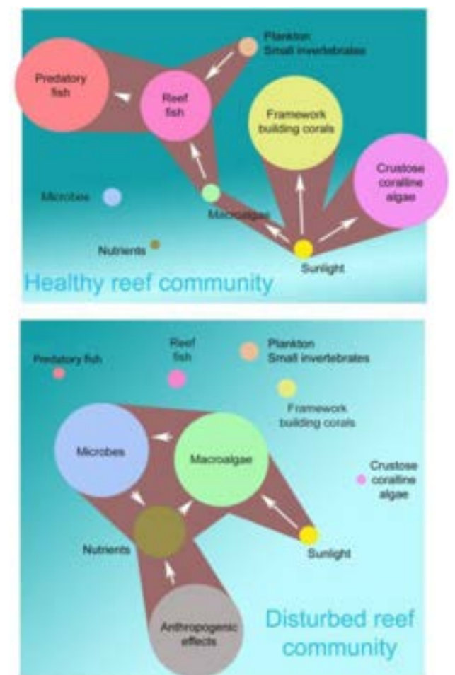
FIGURE 1: Collapse of trophodynamic relationships between functional groups that dominate(d) past and present-day reefs. The shaded area with white arrows indicates the dominant trophic relationships before human disturbance (top) and at present day (bottom).
