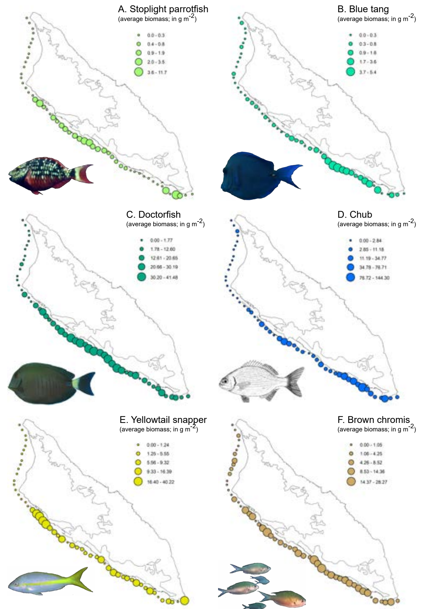
FIGURE 20: Distribution of the 12 most abundant fish species around Aruba (continued on next page).
